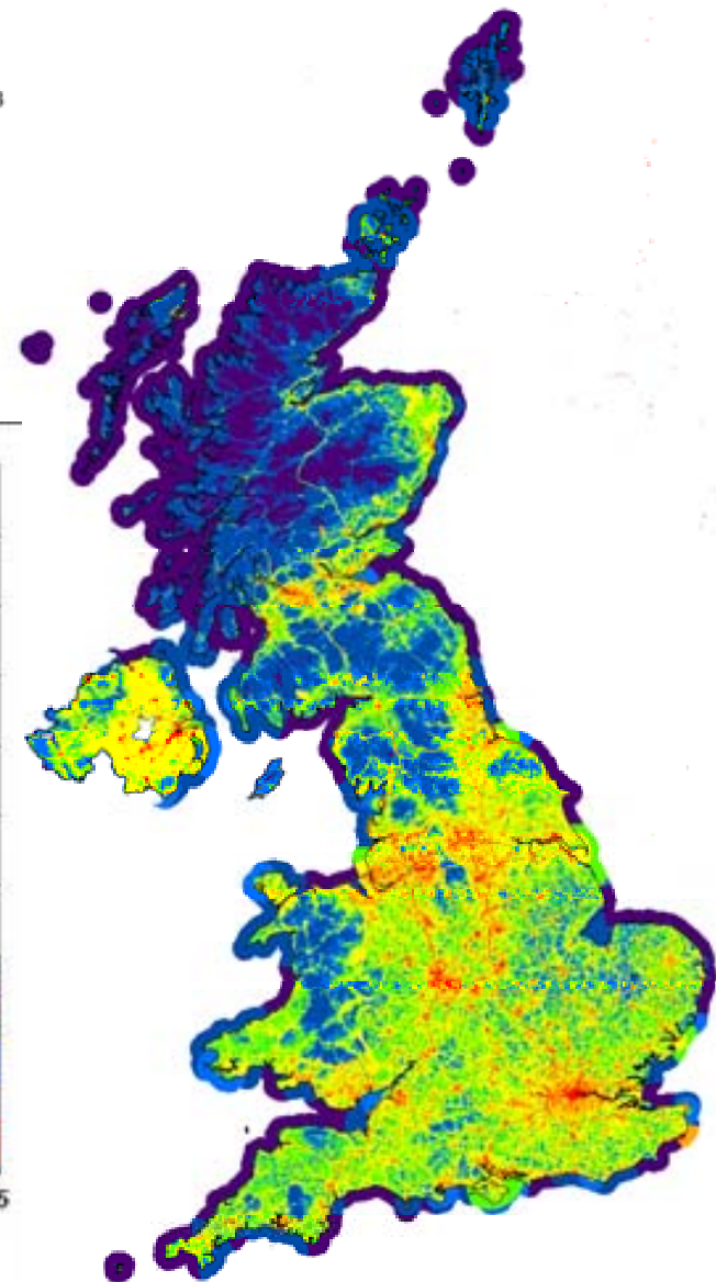
UK Emissions Map of PM 10 2005 t/1x1km
