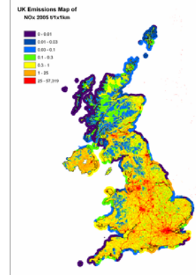
Emission Map for Nitrogen Oxides as NO 2
