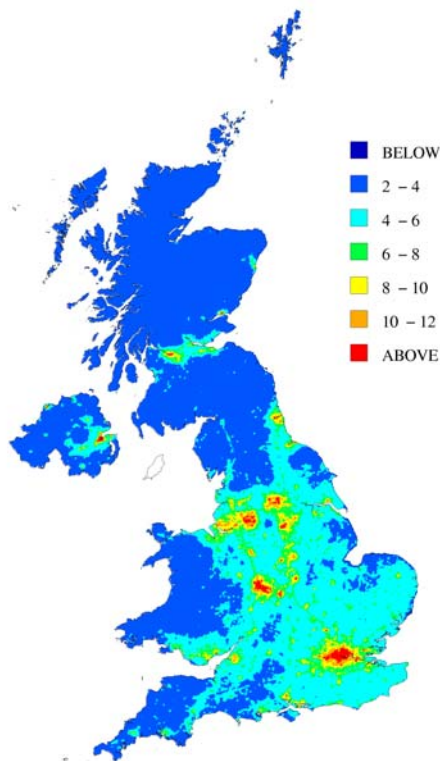
Estimated annual mean background PM 10 concentration, 2006 (ugm-3, gravimetric) primary (including soil and road dusts)
