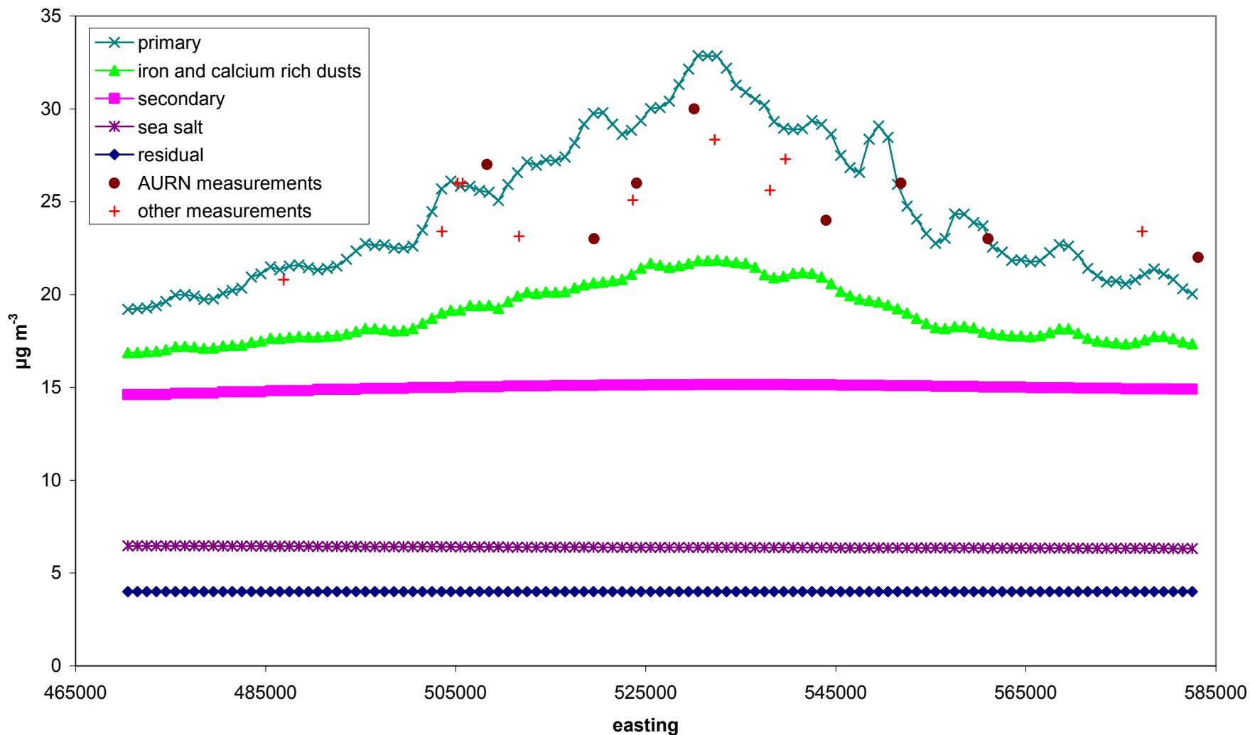
PM 10 transect across London: annual mean 2006 ( \mu\text{g m}^{-3} )
