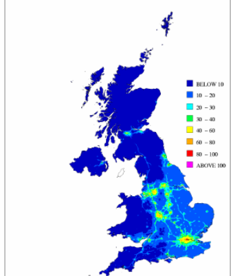
Estimated annual mean background NO x concentration 2004 µg m -3 .
