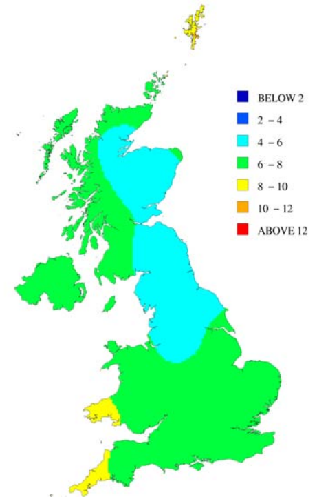
Estimated annual mean background PM 10 concentration, 2006 (ugm-3, gravimetric) sea salt and residual
