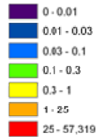
UK Emissions Map of NO x 2005 t/1x1km
