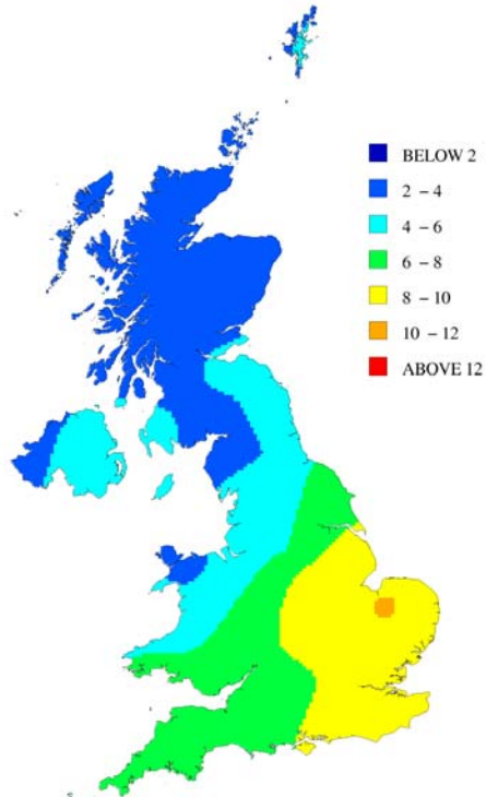
Estimated annual mean background PM 10 concentration, 2006 (ugm-3, gravimetric) secondary inorganic and organic aerosol
