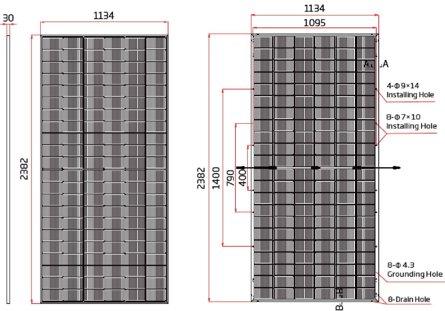
Front View
