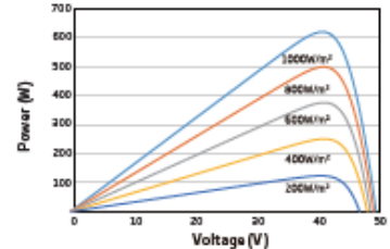
P-V CURVES OF PV MODULE (610W)
