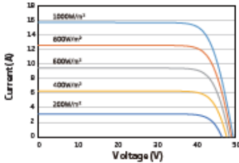
I-V CURVES OF PV MODULE (610W)
