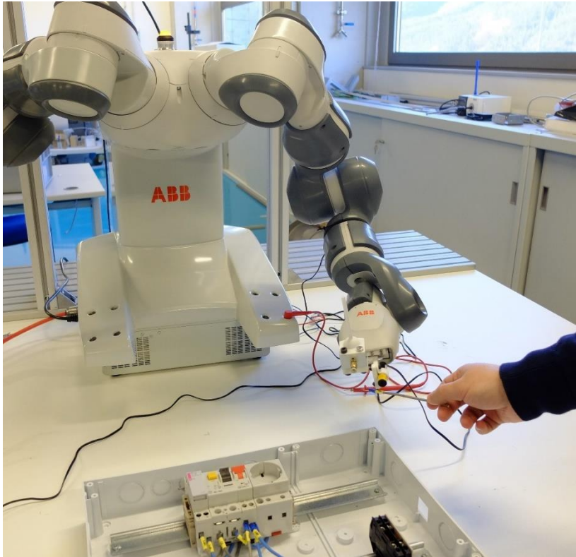
Human operator shows the robot the next cable to be connected
